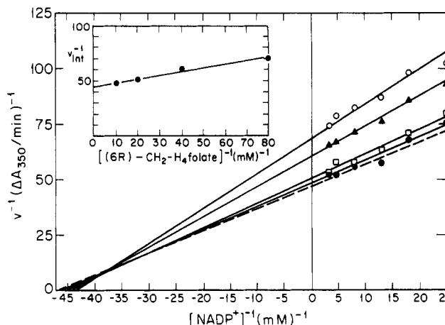
FIGURE 3: Measurement of the steady-state kinetic parameters associated with methylenetetrahydrofolate dehydrogenase activity when (6RS)-CH 2 -H 4 PteGlu 1 is used as the substrate. Double-reciprocal plots of velocity vs. NADP + concentration are shown for (6R)-CH 2 -H 4 PteGlu 1 concentrations of 12.5 (○), 25 (▲), 50 (□), and 100 μM (●). Assays were performed under the conditions described under Experimental Procedures. Each point shown is the average of three to four individual assays. The dashed line represents the extrapolated double-reciprocal plot when (6R)-CH 2 -H 4 PteGlu 1 is present at saturating concentrations. The inset shows a replot of the y-axis intercepts of the double-reciprocal plots vs. (6R)-CH 2 -H 4 PteGlu 1 concentration and was used for the estimation of the position of the dashed line at saturating CH 2 -H 4 PteGlu 1 .
