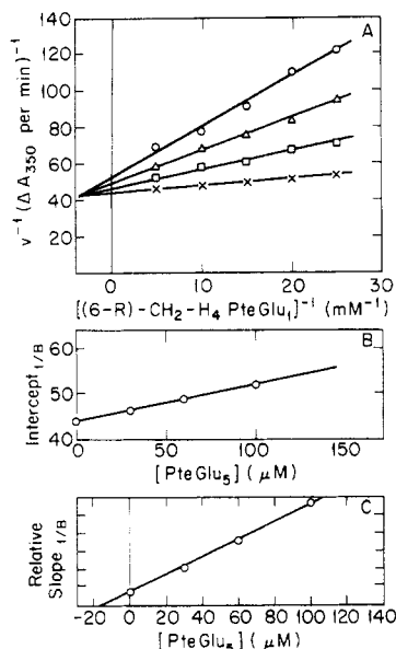
FIGURE 2: Effect of PteGlu 5 on methylenetetrahydrofolate dehydrogenase activity. (A) A double-reciprocal plot of velocity vs. (6R)-CH 2 -H 4 PteGlu 1 concentration in the presence of 0 (×), 30 (□), 60 (Δ), and 100 μM (○) PteGlu 5 . (6R)-CH 2 -H 4 PteGlu 1 was added as the racemic (6RS)-CH 2 -H 4 PteGlu 1 mixture and the NADP + concentration was held fixed at 180 μM. Other conditions are as described under Experimental Procedures. (B) A replot of the y-axis intercepts of the lines in (A) as a function of PteGlu 5 concentration. (C) A replot of the slopes of the lines in (A) as a function of PteGlu 5 concentration.
